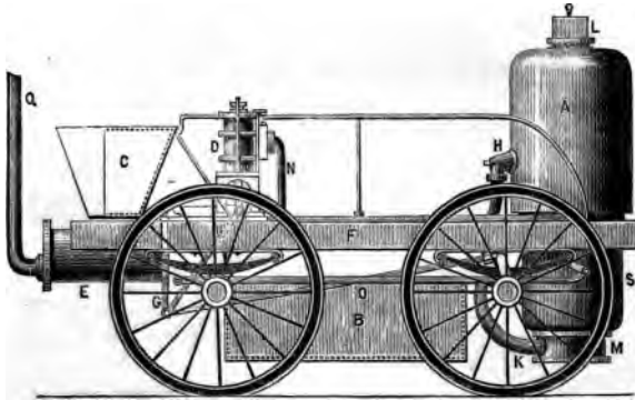
FIG. 54.—The "Novelty," 1829.
